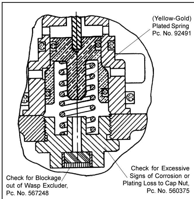
Figure 1 - Part No. 92491 Previous Emergency Limiting Valve Spring
