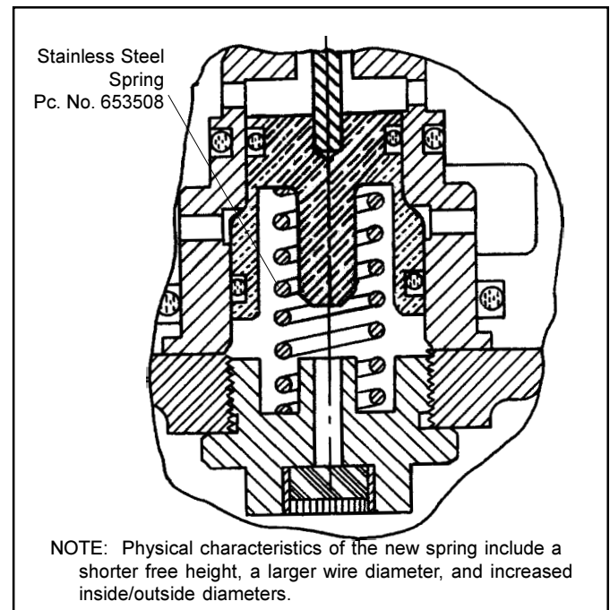
Figure 2 - Part No. 653508 New Stainless Steel Emergency Limiting Valve Spring
